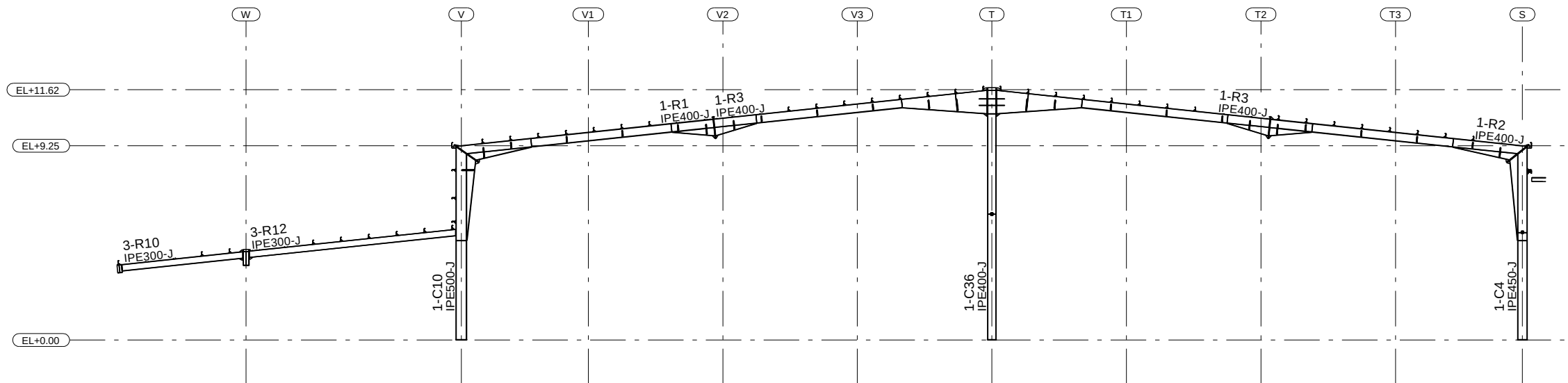
SECTION GRID 3
